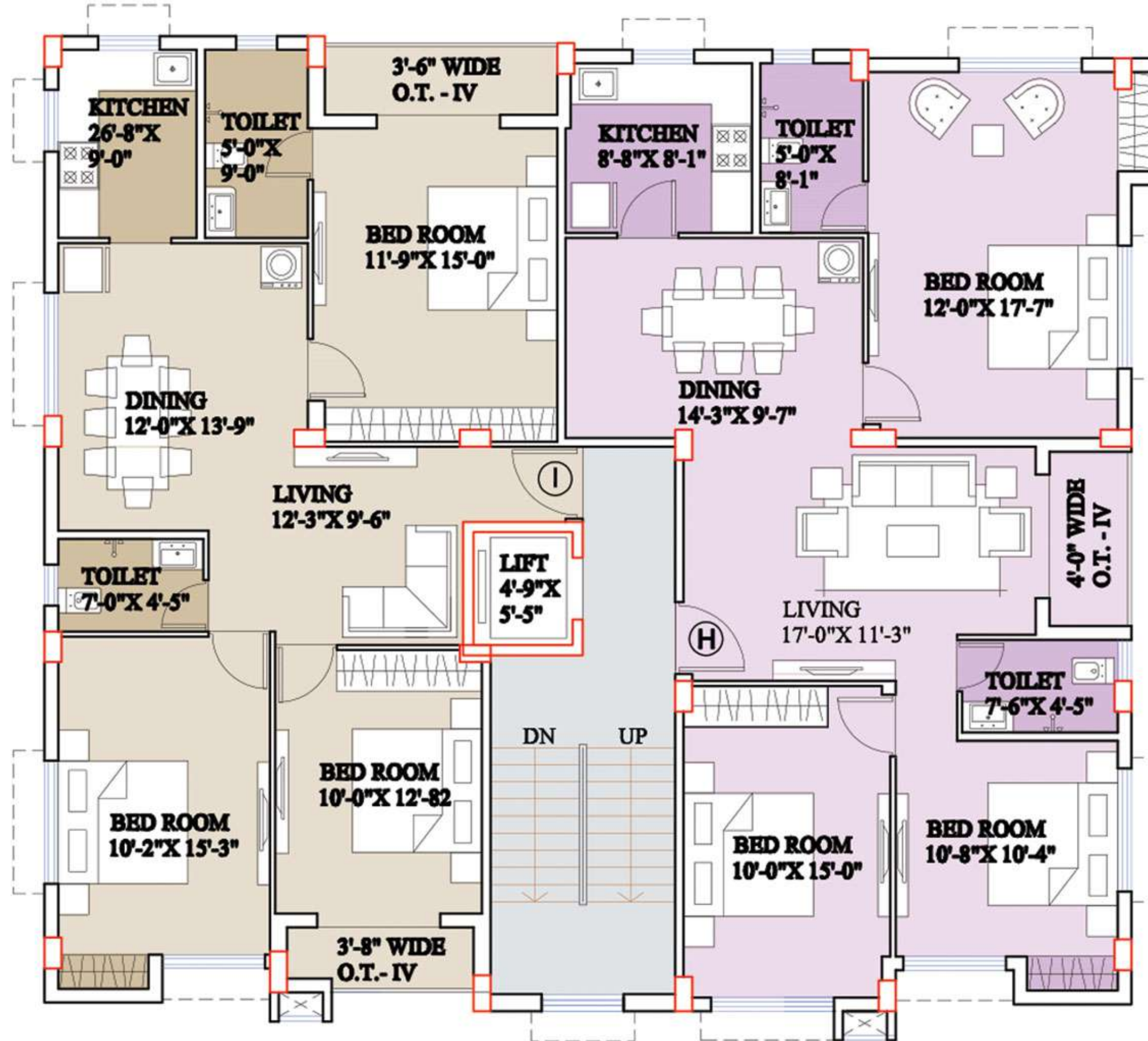
4TH FLOOR PLAN
